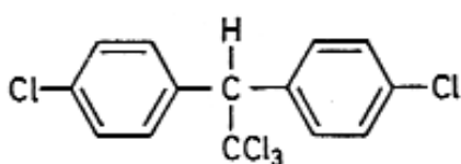
Abb. 1: Dichlor-Diphenyl-Trichlor-ethan (DDT)
